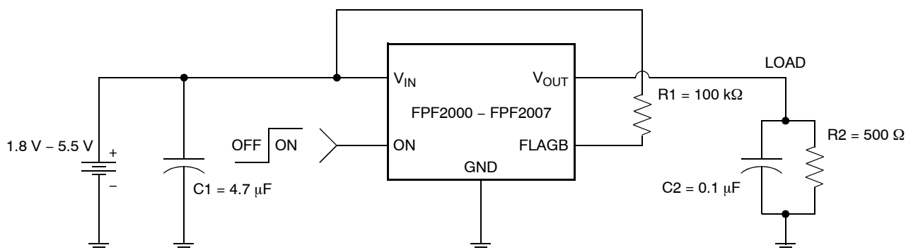
Figure 25. Typical Application
